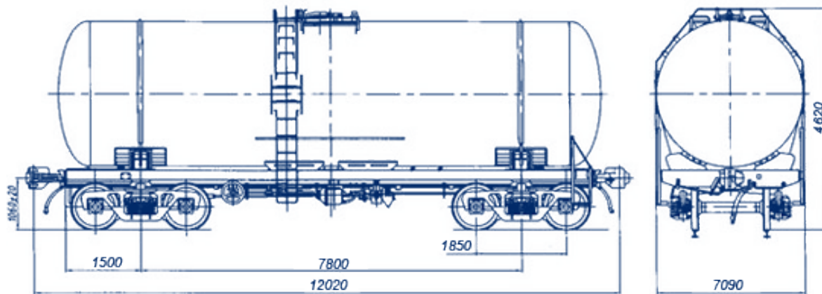
Tank wagon for gasoline and other light oil products model 15-1343-06
