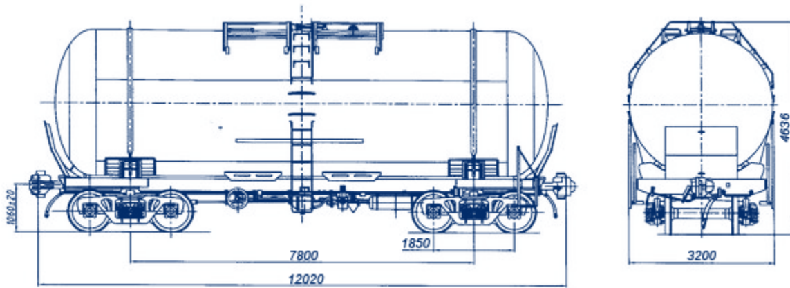
Tank wagon for gasoline and other light oil products model 15-1547-03
