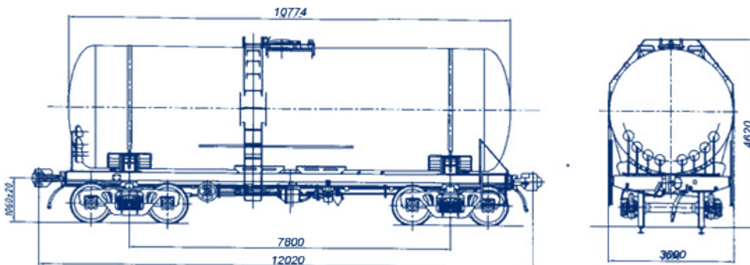
Tank wagon for viscous oil model 15-1566-07
