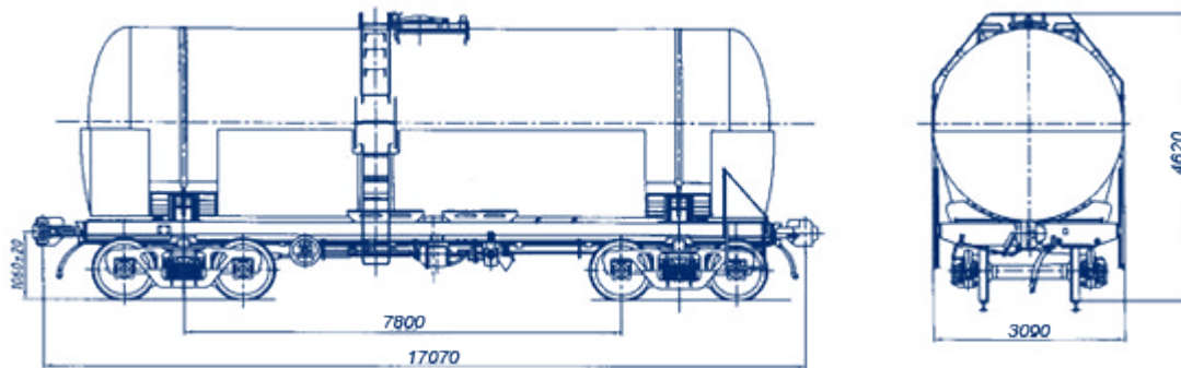
Tank wagon for viscous oil model 15-1566-06
