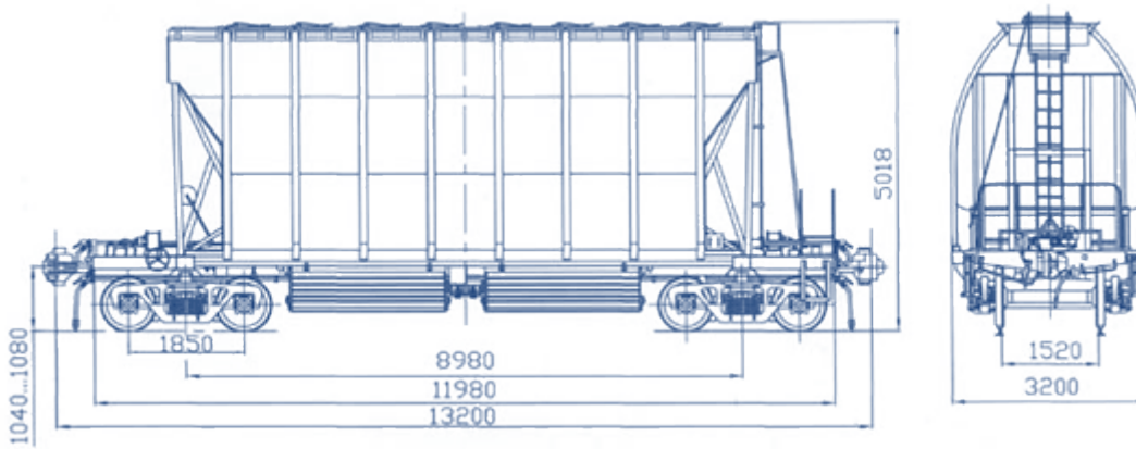
Wagon-hopper for powdered model 19-1761
