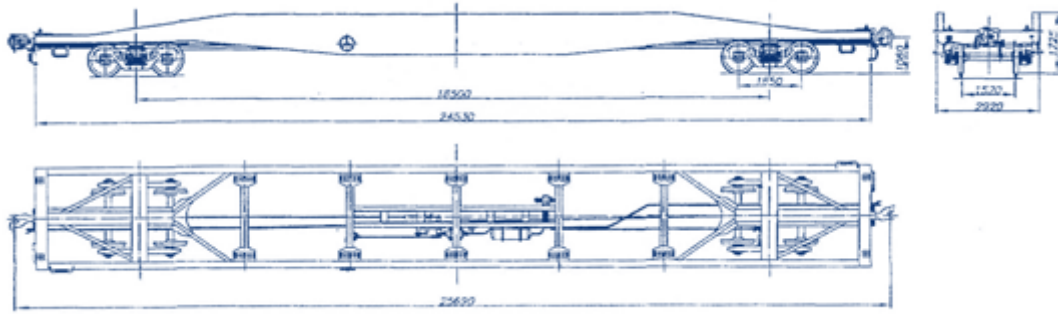
Wagon-platform for high-capacity containers, model 13-1796
