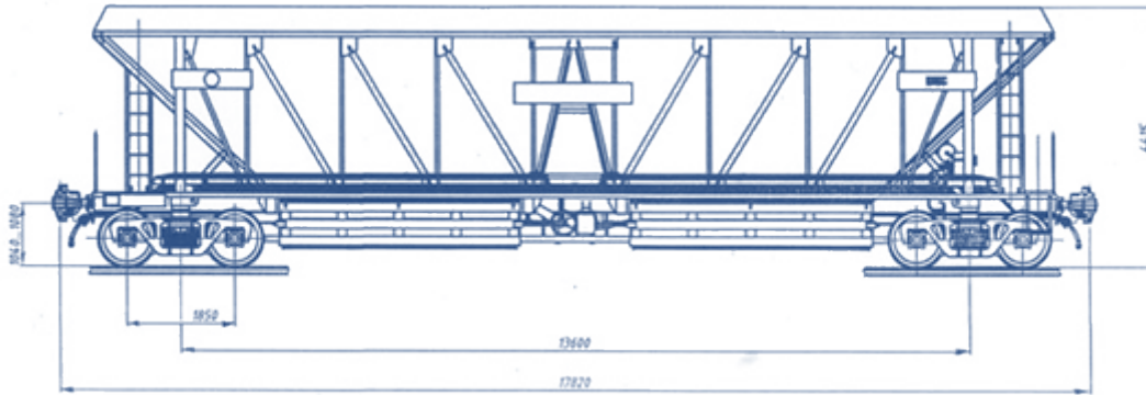
Wagon-hopper for refrigerated Coke, model 22-1764
