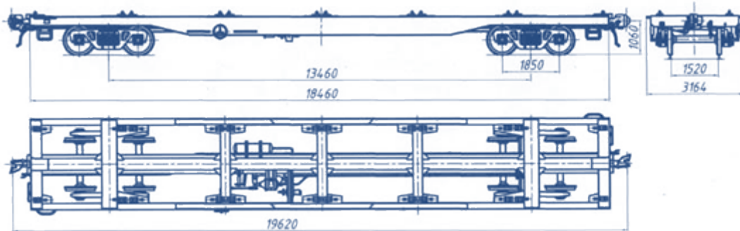
Wagon-platform for high-capacity containers, model 13-1798
